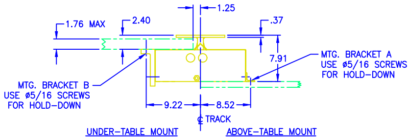
TRACK MTG. DETAIL ENLARGED VIEW
