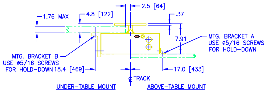
TRACK MTG. DETAIL ENLARGED VIEW
