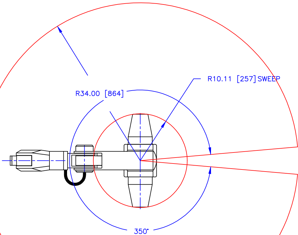
Plan View Dimensions - Inches[mm] A460 ROBOT ARM
