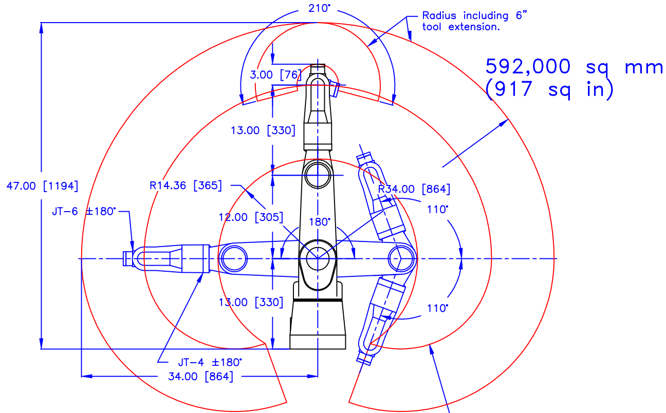
Elevation DIMENSIONS IN Inches [mm] A460 ROBOT ARM
